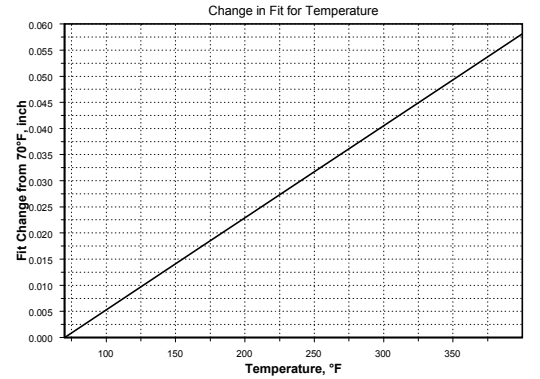
206R4530 Roper 2-1/16" 3 Stage 4/5 Power Section
