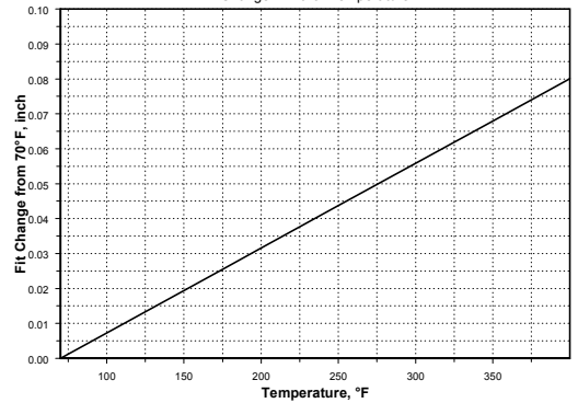
206R1220 Roper 2-1/16" 1/2 2 Stage Power Section Change in Fit for Temperature
