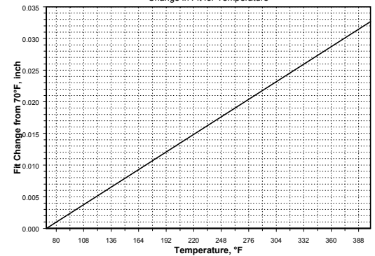
206R5630 Roper 2-1/16" 5/6 3 Stage Power Section Change in Fit for Temperature
