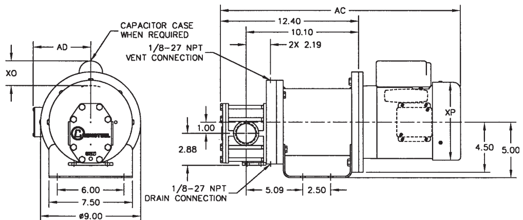
SM9 MAG DRIVE W/ FOOT ACCESSORY DIMENSIONS
