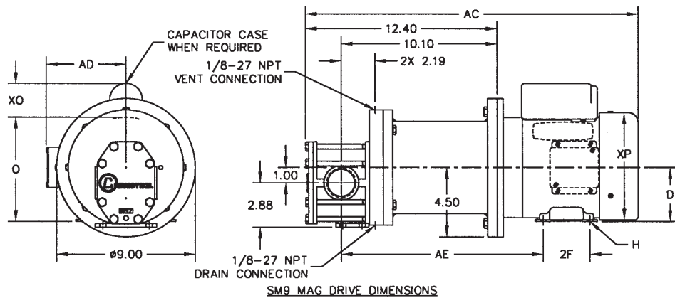
SM9 MAG DRIVE DIMENSIONS
