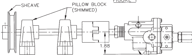
STANDARD N1000L(R) SERIES PUMP FIGURE 2
