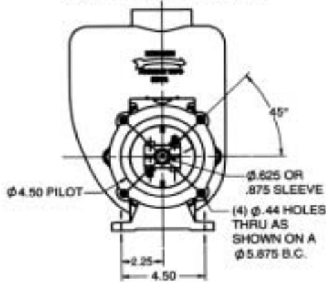
PUMPAK FOR ELECTRIC MOTOR
