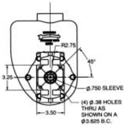
PUMPAK FOR ENGINE
