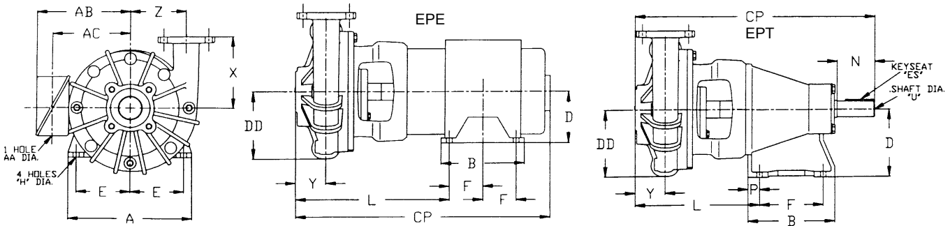
EPE20K2H 3600 RPM ODP - DIMENSIONS MEASURED IN INCHES
