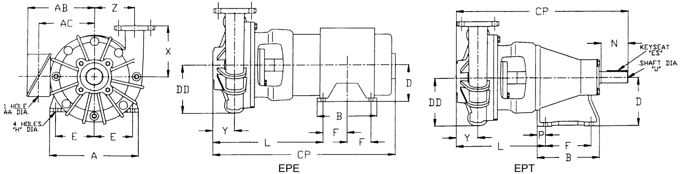
EPE12K1H 3600 RPM ODP - Dimensions measured in inches
