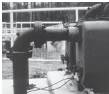
Settling Pond
