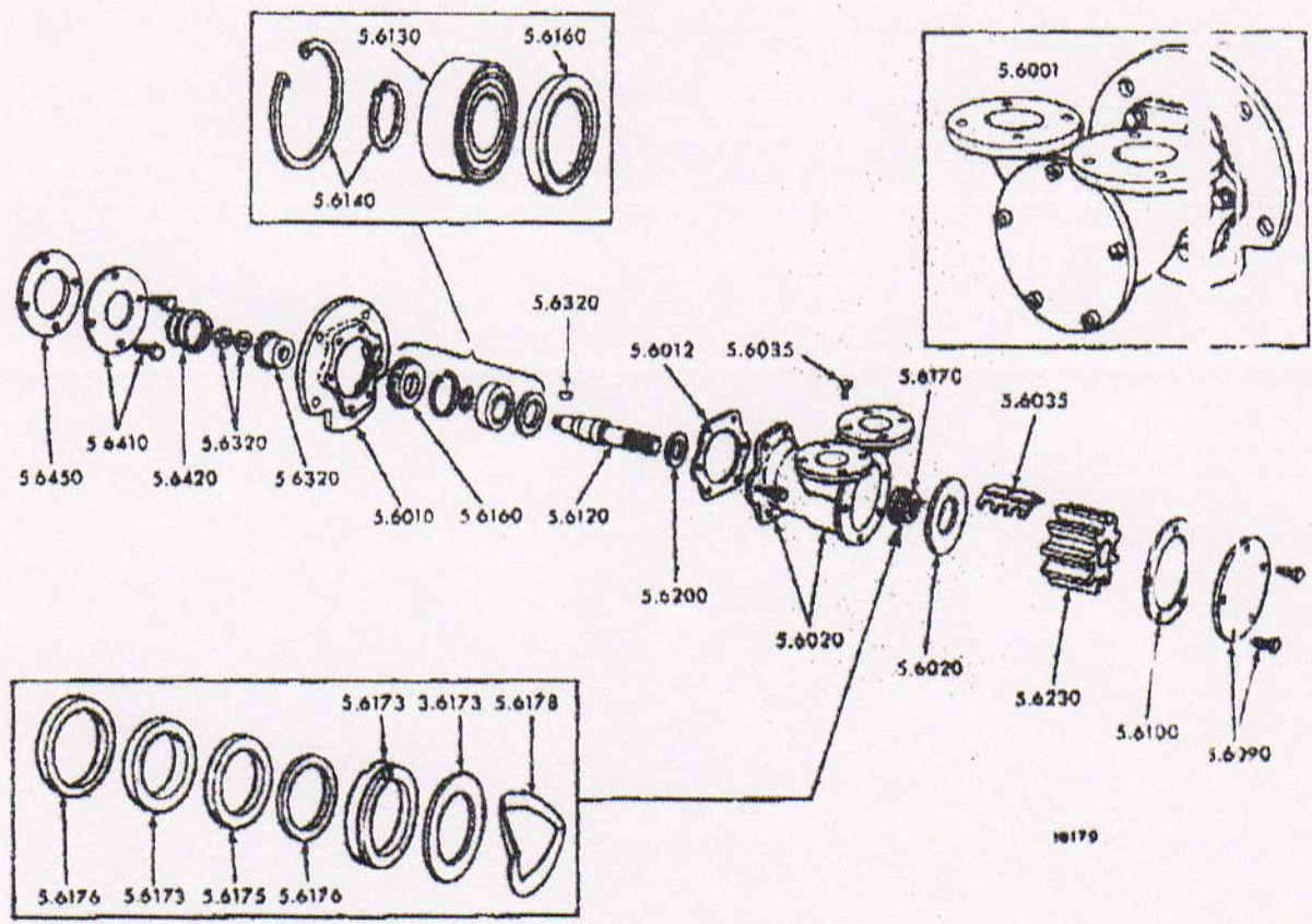
FIG. 8B RAW WATER PUMP (V-Models)
