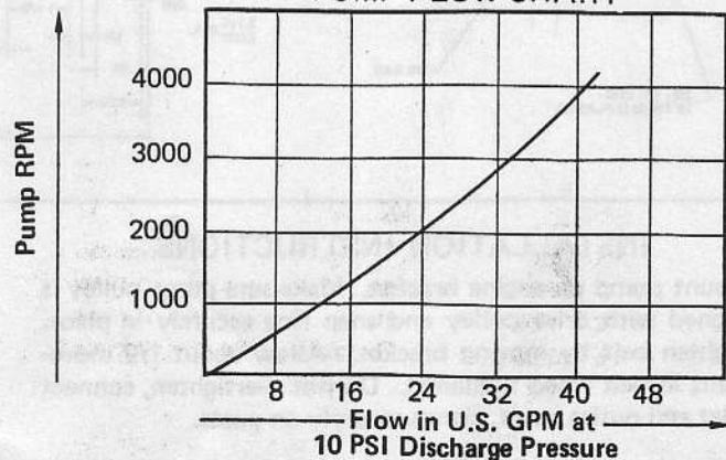
PUMP FLOW CHART
