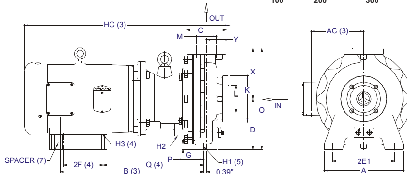
Dimensions (inches) and Specifications Note: Will vary by motor manufacturer
