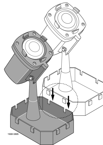
Figure 3 - Typical Multiple Light Installation.
