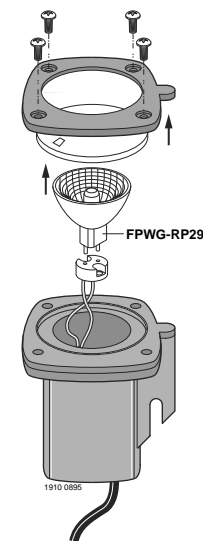
Figure 4 - Bulb Replacement.
