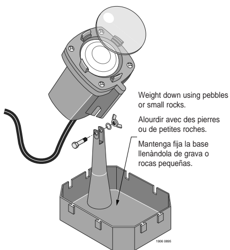
Figure 1 - Typical Installation Using Base.
