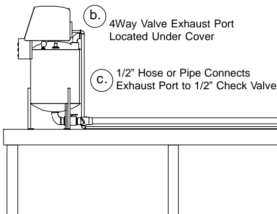
fig 16 Positive Head Vacuum Exhaust Plumbing
