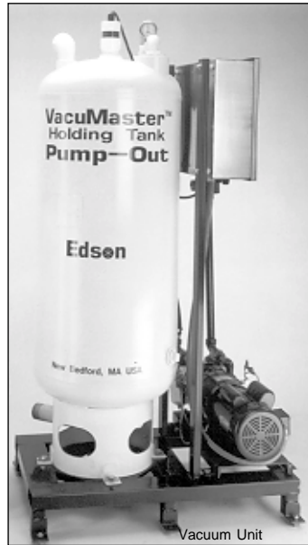
Vacuum Unit
