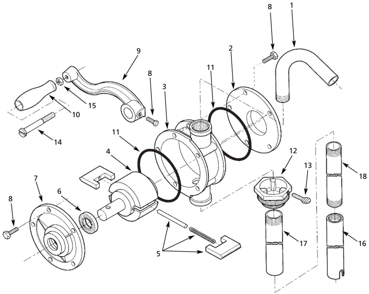
Figure 1 – Repair Parts Illustration
