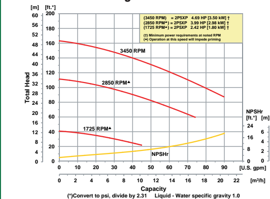
Performance of 2" High Pressure Pedestal Pumps
