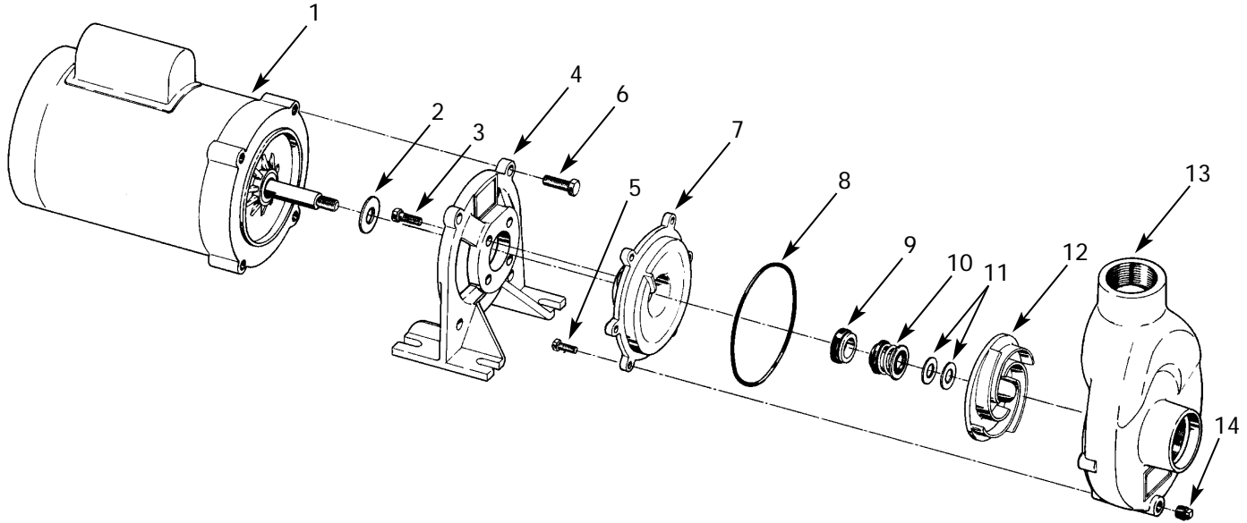
Figure 2 - Repair Parts Illustration
