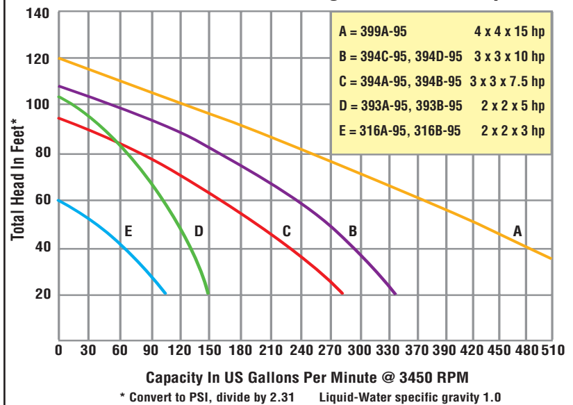
Performance of Sewage & Trash Pump
