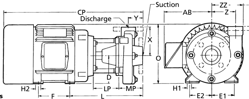
Figure 1 - Dimensions
