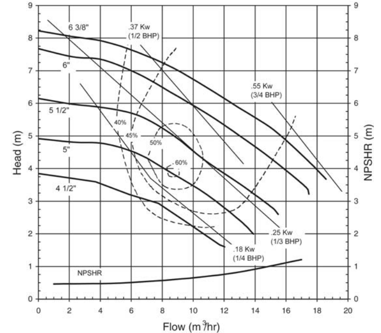
50 Hz 1450 rpm
