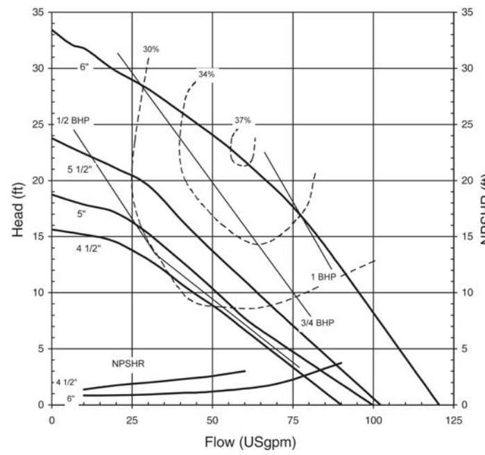
60 Hz 1725 rpm
