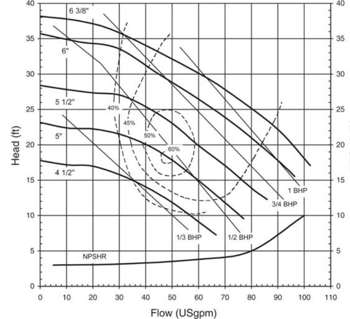
60 Hz 1725 rpm
