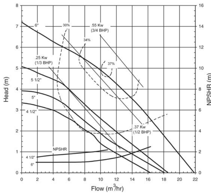
50 Hz 1450 rpm
