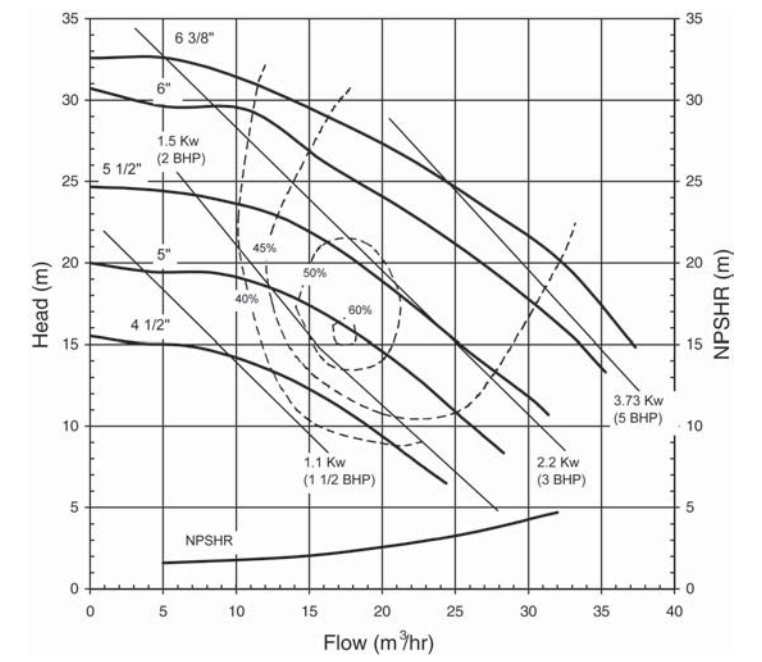
50 Hz 2900 rpm
