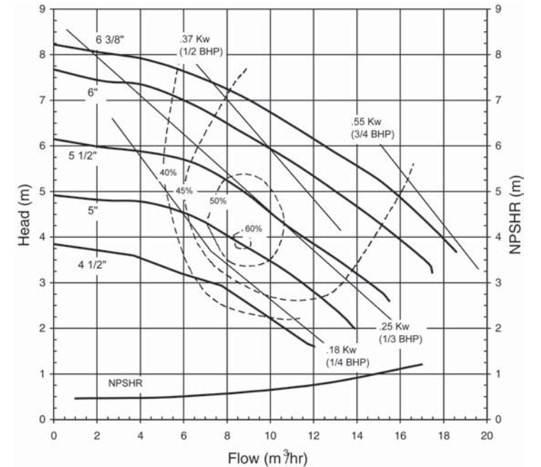
50 Hz 1450 rpm
