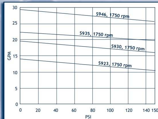
S923, S930, S935 and S946 Series
