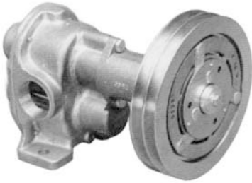
N11HDM, N13HDM Clutch
