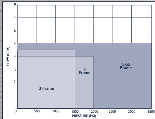
Mid-Size Industrial Plunger Pumps
