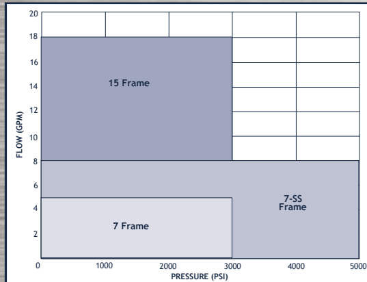
High Pressure Intermediate Size Industrial Pumps
