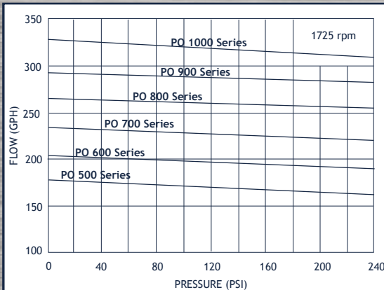
Series 500 - 1000 High Volume Clamp / Flange Mount
