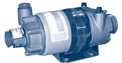
101 Series (3/8" Ports) Miniature Stainless Steel Pump
