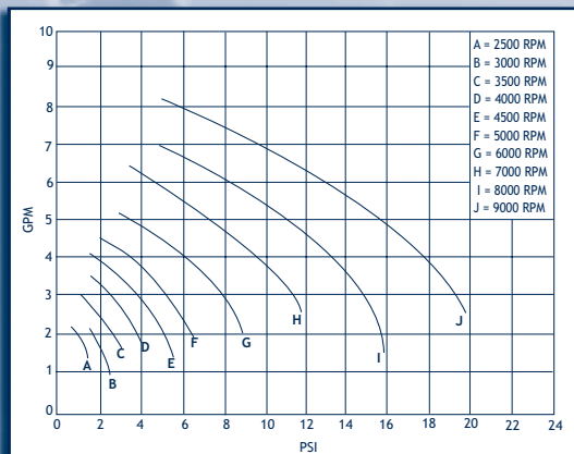
101 Series (3/8" Ports) Miniature Stainless Steel Pump
