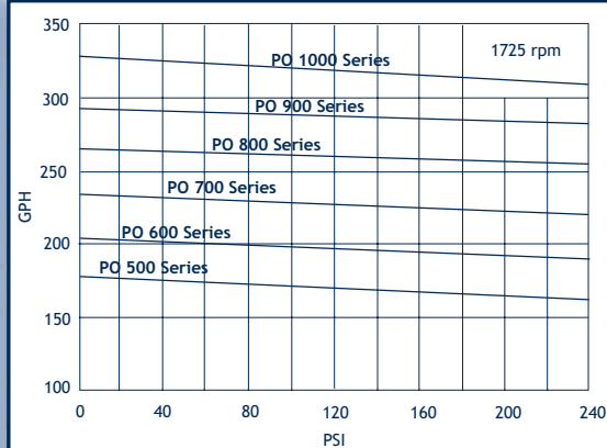
Series 500 - 1000 High Volume Clamp / Flange Mount
