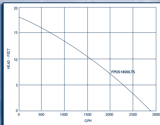
10 gal. Effluent/Water Sump
