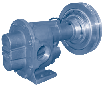
Clutch Driven
