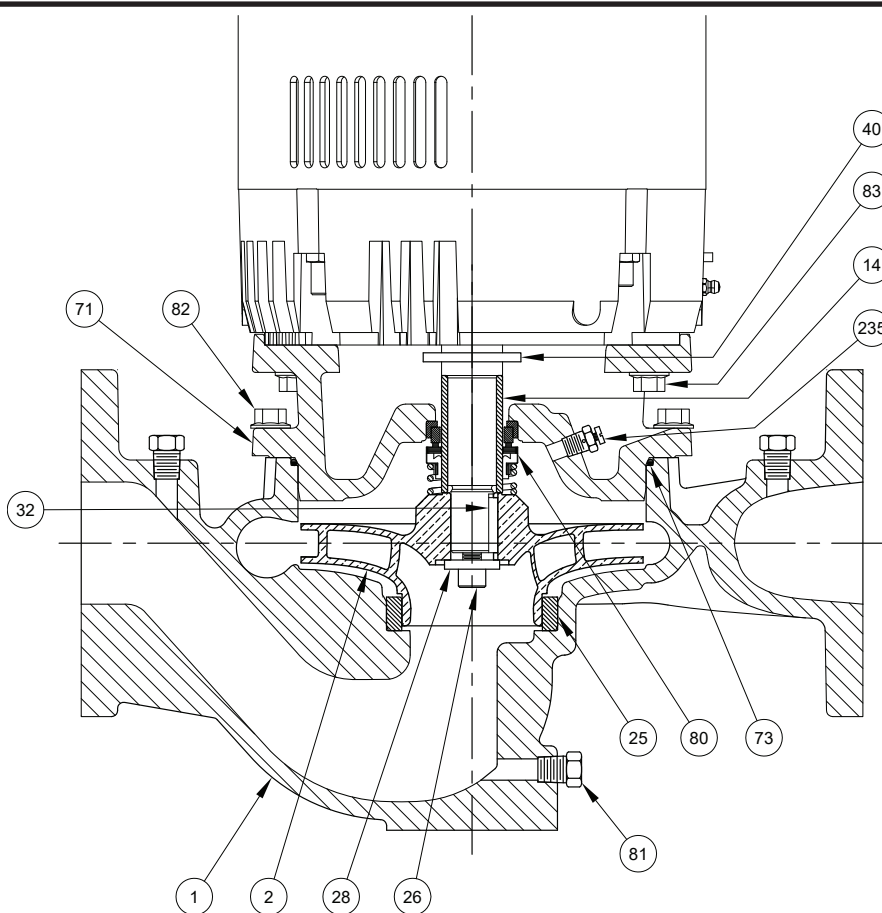
Parts List and Materials of Construction Standard Casing Working Pressure - 175 PSI @ 100° F
