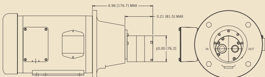
D90 IEC 1.5 kW MOTOR
