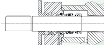
Shaft sealing GP (typ. application: bitumen processing)
