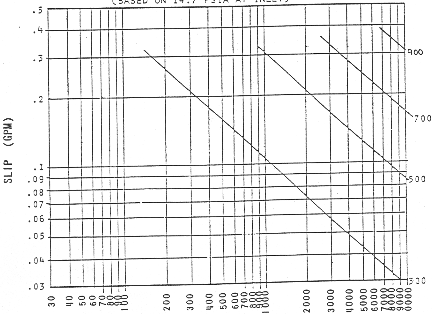
GRAPH II (BASED ON 14.7 PSIA AT INLET)
