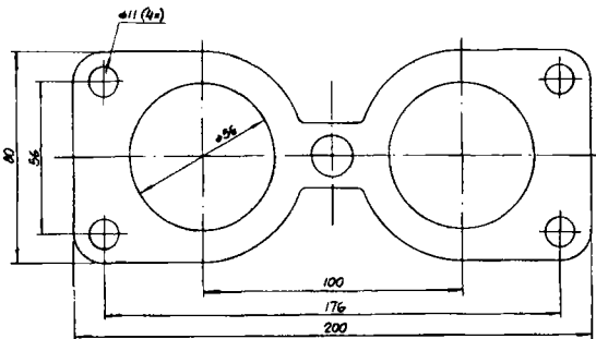
F9B-9 Impeller Pump Art. No. 10-13080-01
