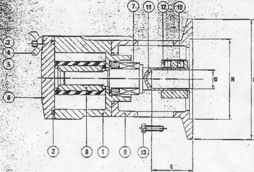
CROSS SECTION
