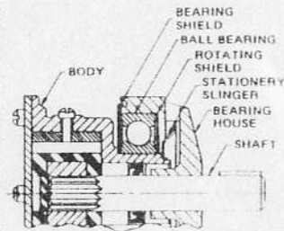
Cross Section to show relative position of bearing and slinger parts
