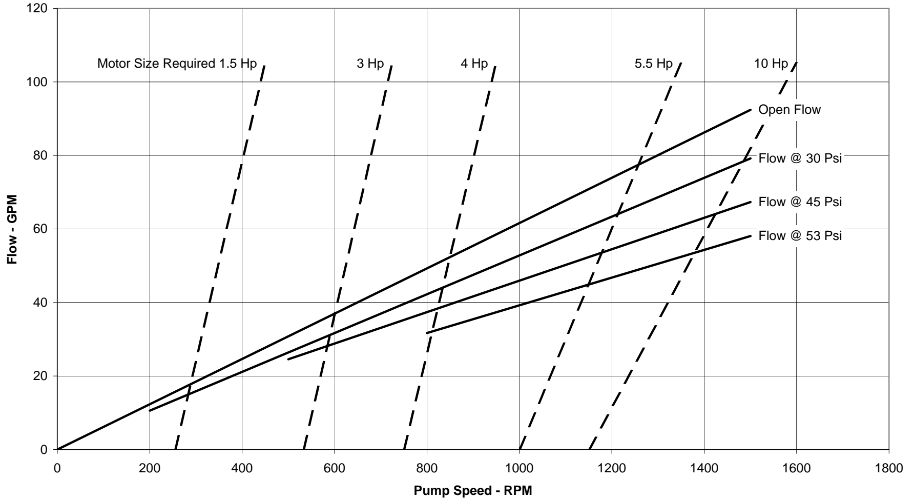
30540/30580 Series Performance Curve - High Pressure FG Neoprene Impeller Viscosity 500 - 2000 Cp - Starting Torques Fwd 27.2 lbf-ft / Rev 48.5 lbf-ft
