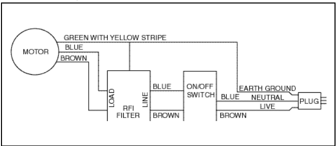
WIRING DIAGRAM 16450-3220, 2220
