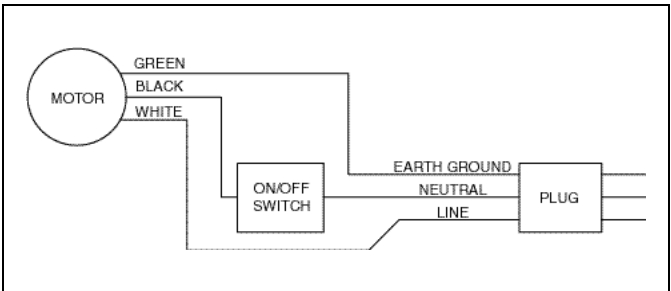
WIRING DIAGRAM 16450-0115
