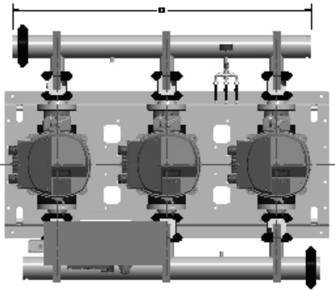
208-230V AquaForce e-HV Dimensions 15SV - 3 Pump
