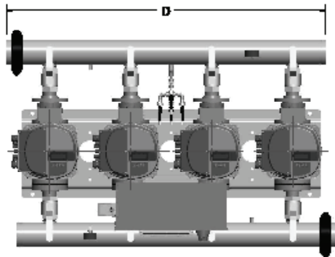
208-230V AquaForce e-HV Dimensions 10SV - 4 Pump
