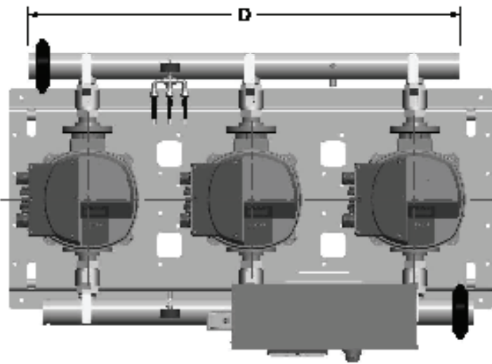
208-230V AquaForce e-HV Dimensions 10SV - 3 Pump
