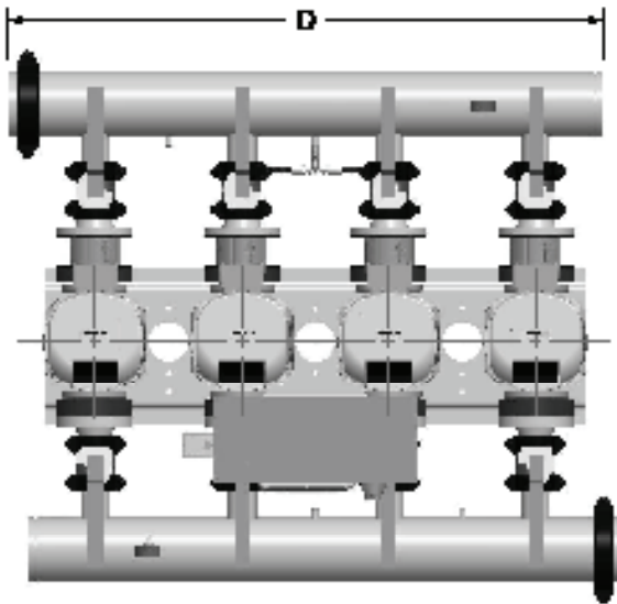
460V AquaForce e-HV Dimensions 15SV - 4 Pump
