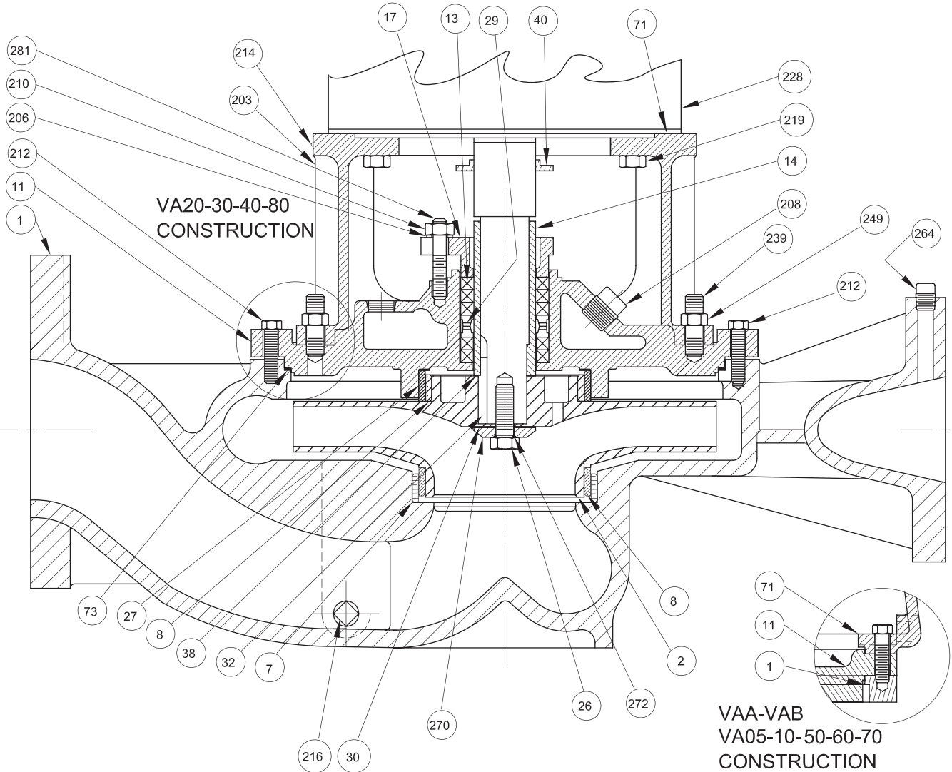
Optional Construction with Water Jacketed Stuffing Box
