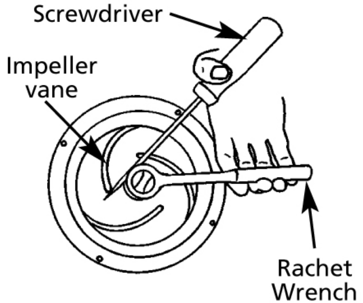
Figure 1 - Impeller Removal
